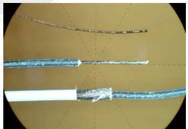
Comparison: Microcoax cable / human hair
