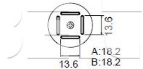
A1180B BQFP 17 x 17
