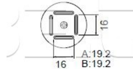
A1181B BQFP 19 x 19
