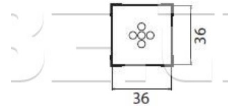
A1476 BGA 35 x 35
